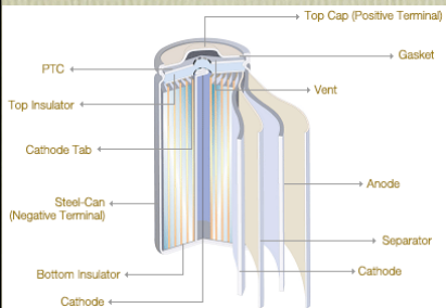
Spiral Wound Cylindrical Cell
