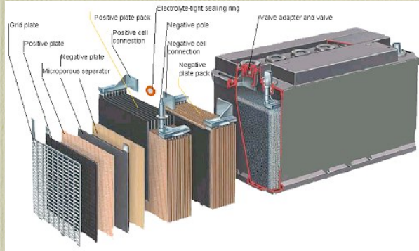
Common automobile battery
