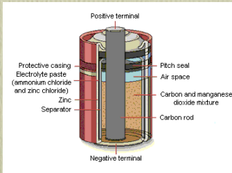
“flash light” battery
